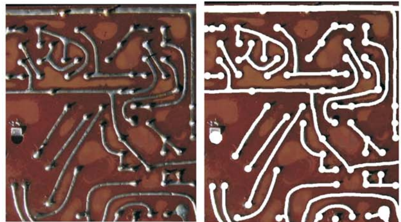
5. Magnify, crop, and mask traces to white for color separation.
